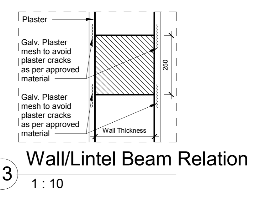
13 Wall/Lintel Beam Relation 1 : 10
