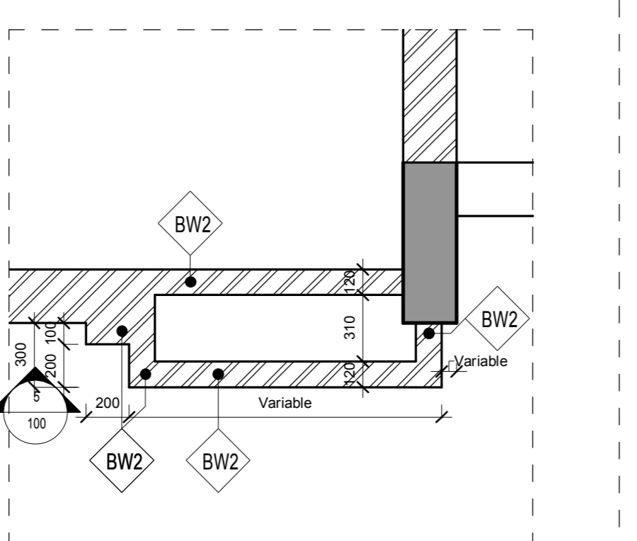
4 Blockwork/Column Detail 3 1 : 25
