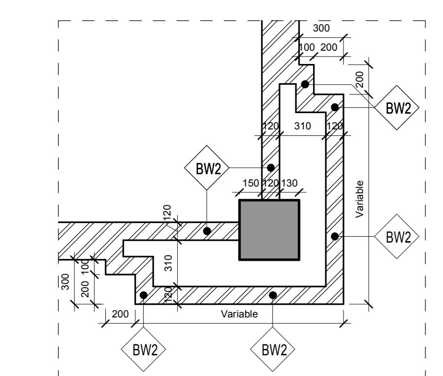
2 Blockwork/Column Detail 1 1 : 25
