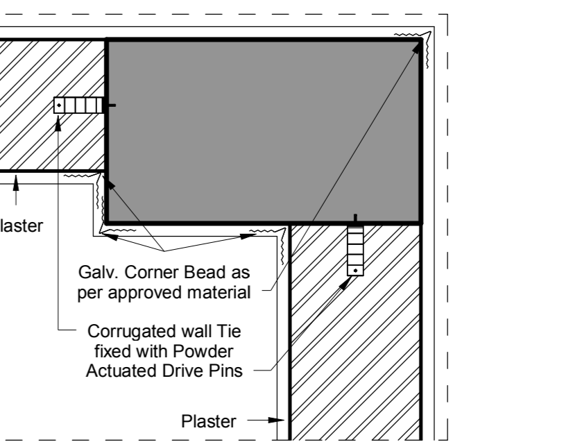
15 Wall/Column Relation 1 : 10
