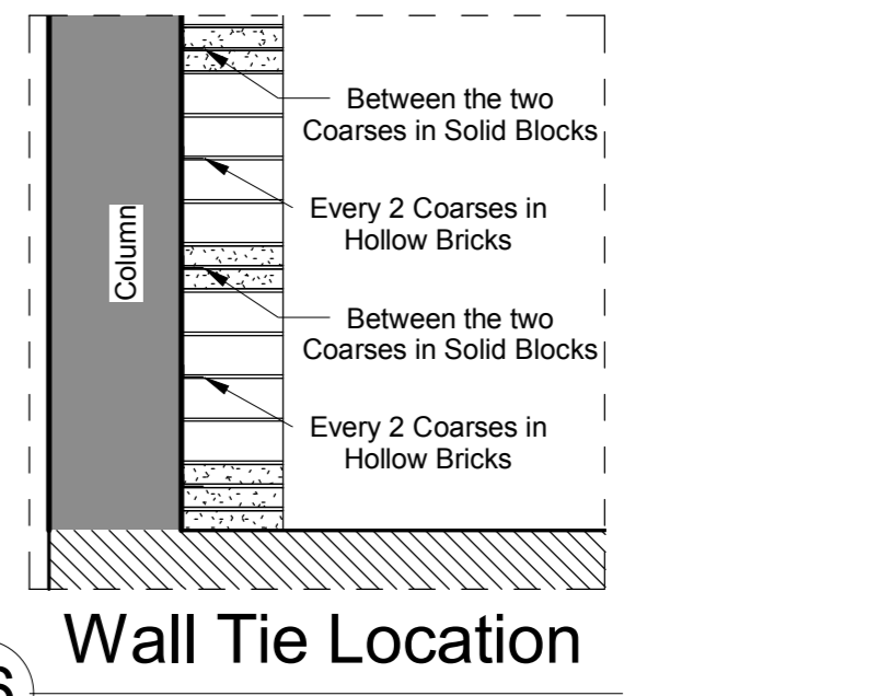
16 Wall Tie Location 1 : 25
