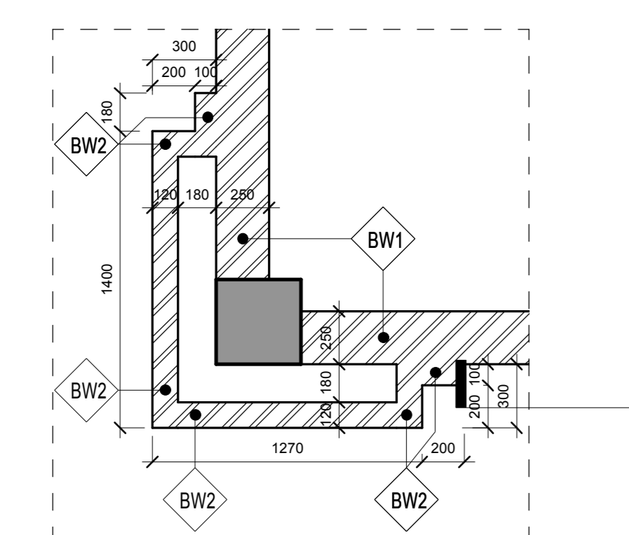
3 Blockwork/Column Detail 2 1 : 25
